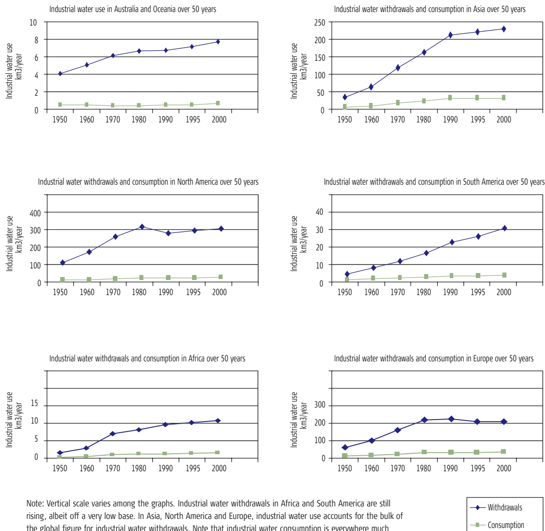
Figure 8.1: Trends in industrial water use by region, 1950-2000
